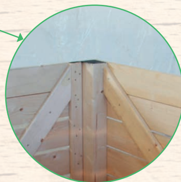
Detail of the inside - side log
